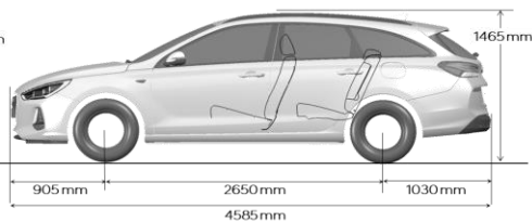
Wagon
