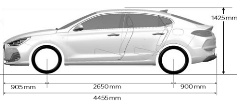
Fastback
